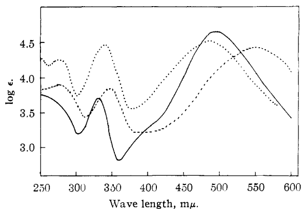
Fig. 2.—Absorption spectra of benzhydryl carbonium ions in 100% sulfuric acid: —, hexamethyl (0.0133 g. of ether per liter); ·····, decamethyl (0.0091 g. of carbinol per liter), - · - ·, octamethyl (0.0170 g. of carbinol per liter).
